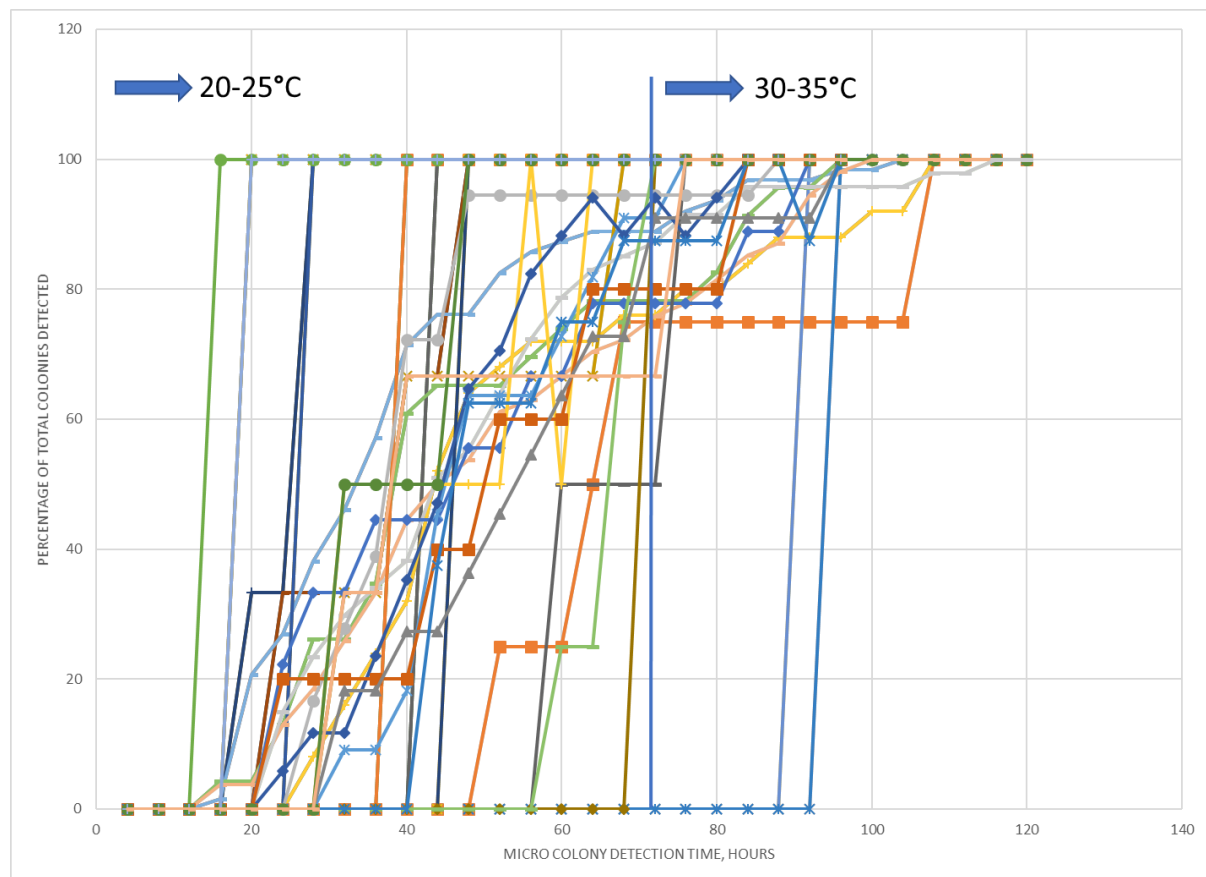
Figure 3. TTR profiles for multiple sample types with serial incubation for 3 days 22.5°C then 2 days 32.5°C
