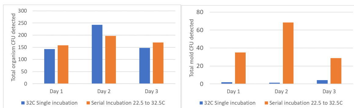
Figure 2a Total organism recovery compared using two incubation strategies
