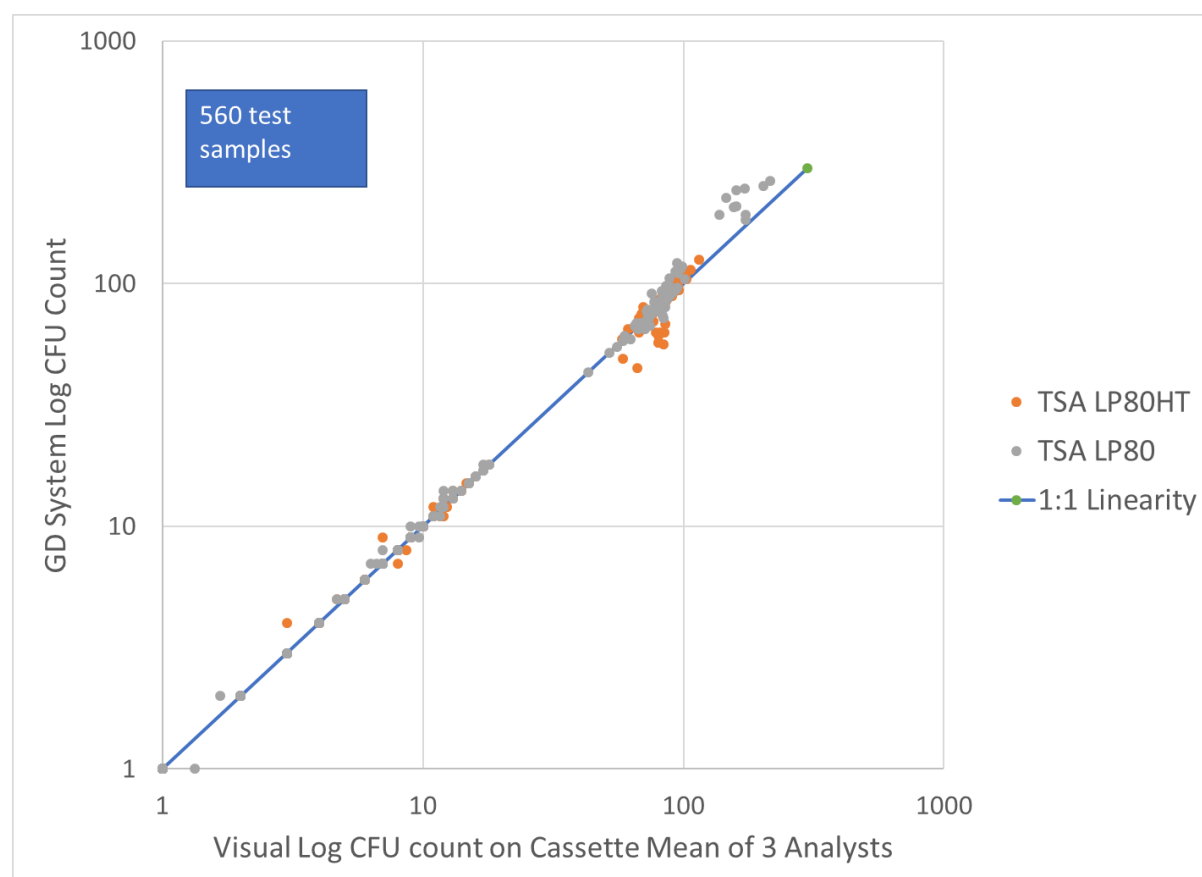
Figure 1 Correlation of System CFU counts compared to the mean CFU count of 3 analysts on the same cassette.
